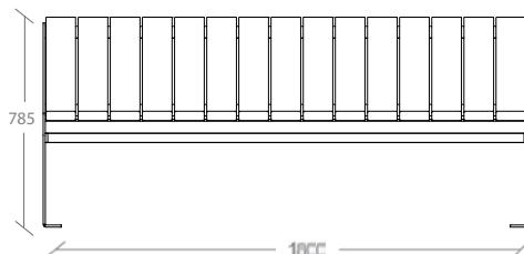
▲ Mod. C-1002-M-OX Acero pintado / steel powder coated with oxiron paint / acier pient noir
