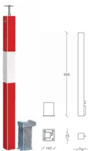
▲ PARKING EXTRAIBLE Mod. P-E
